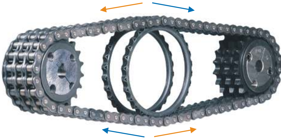
ROLL-RING (PO -P )
